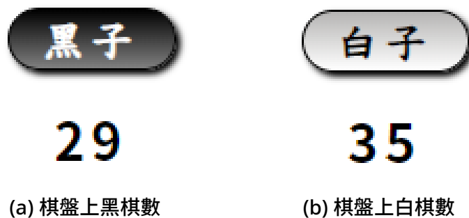
Figure 11: 棋子狀態
